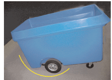
Wheel Placement Provides Ideal Leverage for Control & One Person Dumping
