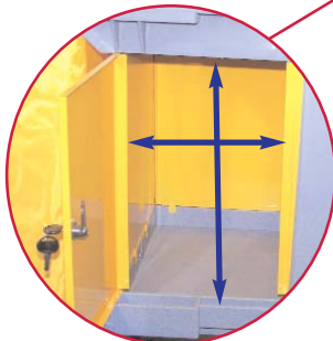
#6156 Lockbox Large 8½" x 14" entry 205 cubic inches of storage Unbreakable 19 gauge Steel
